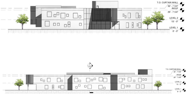
BUILDING ELEVATIONS
